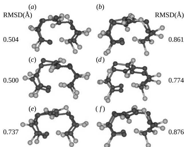
Figure 9. Superpositions of nine equivalent atoms (only C^\beta of the \beta -residue is omitted) of observed \alpha\beta/\beta\alpha -turns with their \alpha -peptide type I and type II turn counterparts (ideal structures). Superposition of (a) type I \beta -turn and \alpha\beta (1) turn of Boc-(Aib- trans ACPC) _4 OBz, (b) type II \beta -turn and \alpha\beta (1) turn of Boc-(Aib- trans ACPC) _4 OBz, (c) type I \beta -turn and \beta\alpha (1) turn of Boc-(Aib- trans ACPC) _4 OBz, (d) type II \beta -turn and \beta\alpha (1) turn of Boc-(Aib- trans ACPC) _4 OBz, (e) type I \beta -turn and \alpha\beta -turn of molecule B of Boc-Aib- \beta -Res-Aib-OMe and (f) type II \beta -turn and \alpha\beta -turn of molecule B of Boc-Aib- \beta -Res-Aib-OMe ( \beta -Res in E and F=8-aminocyclooct-4-ene carboxylic acid).
