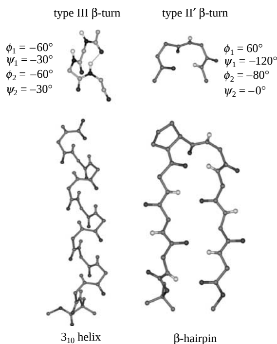
Figure 10. Nucleation of helices and hairpins by local turn formation in \alpha -polypeptide structures. Turns shown are idealized structures. The helix is a view of pBrBz-(Aib) _{11} -OtBu (Gesman et al. 2003). The average \phi , \psi values for the 3_{10} -helix are -52.4^\circ and -31.1^\circ . The hairpin is from the structure of Boc-Leu-Val-Val-DPro-Gly-Leu-Val-Val-OMe (Karle et al. 1996). The \phi , \psi values at the turn residues are: \phi_{(i+1)}=62.5^\circ , \psi_{(i+1)}=-132.4^\circ , \phi_{(i+2)}=-80.7^\circ and \psi_{(i+2)}=-3.4^\circ . Side-chain atoms of the residues and protecting groups in the helix and hairpin have been deleted for clarity.
