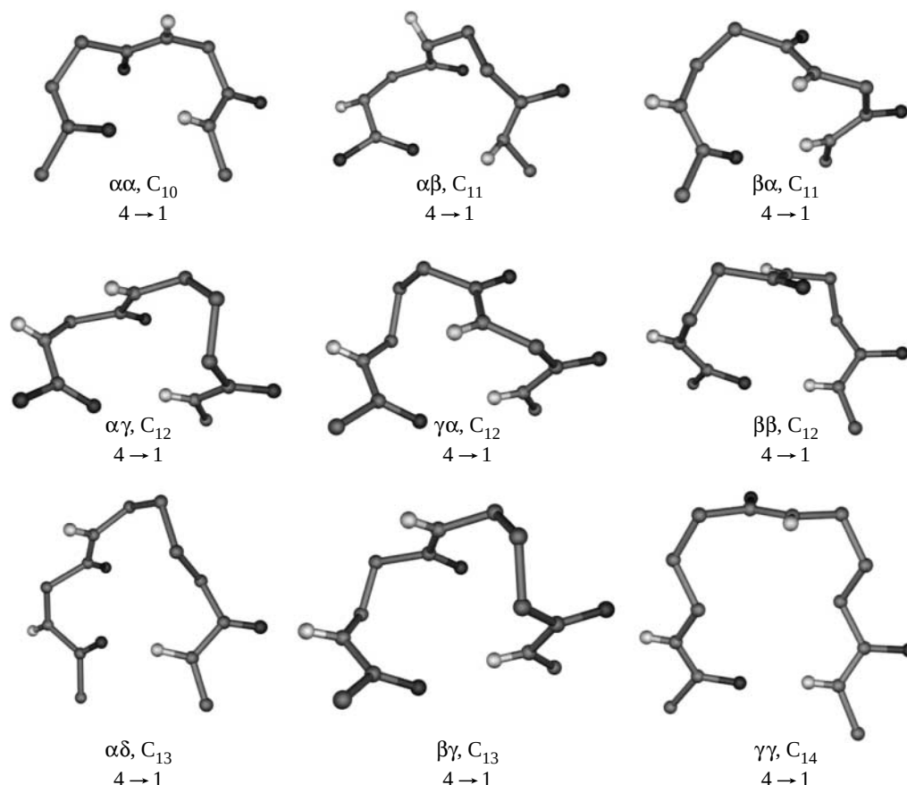
Figure 7. Examples of turn structures (normal hydrogen-bond direction) characterized by X-ray diffraction, \alpha\alpha , Boc-Leu-Phe-Val- p Pro-Gly Leu-Phe-Val-OMe (Karle et al. 1996); \alpha\beta , Boc-Aib-Aib- \beta Gly NHMe (Pavone et al. 1992); \beta\alpha , Boc-Val-Ala-Phe-Aib- \beta Val- \beta Phe-Aib-Val-Ala-Phe-Aib-OMe (Roy et al. 2004); \alpha\gamma , Boc-Aib-Gpn-Aib-Gpn-OMe (Ananda et al. 2005); \gamma\alpha , Boc-Aib-Gpn-Aib-Gpn-OMe (Ananda et al. 2005); \beta\beta , Boc-( trans ACPC) 8 -CO 2 CH 2 Ph (Appella et al. 1999c); \alpha\delta , Boc-Leu-Val-Val- p Pro- \delta Ava-Leu-Val-Val-OMe (Rai et al. in press); \beta\gamma , Boc-Leu-Aib-Val- \beta Gly \gamma Abu-Leu-Aib-Val-OMe (Karle et al. 1997); \gamma\gamma , Boc- \gamma -ResA- \gamma -ResB-NHMe ( \gamma -ResA=2 benzyl, 4 methyl- \gamma -aminoisobutyric acid, \gamma -ResB=4 isopropyl, 2 methyl \gamma aminoisobutyric acid; Brenner & Seebach 2001).
